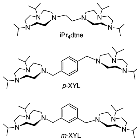
Fig. 5. Binucleating ligands used to explore \text{Cu}^{\text{I}}/\text{O}_2 chemistry [15,17].
