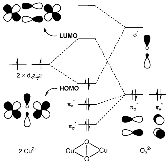
Fig. 2. Partial molecular orbital diagram showing the frontier orbitals of the (\mu\text{-}\eta^2\text{:}\eta^2\text{-peroxo})\text{dicopper(II)} core, adapted from [3,6].
