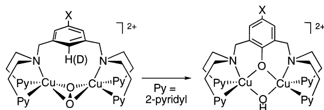
Fig. 8. Hydroxylation of an arene by a bent ( \mu\text{-}\eta^2\text{:}\eta^2\text{-peroxo} )dicopper complex [24].
