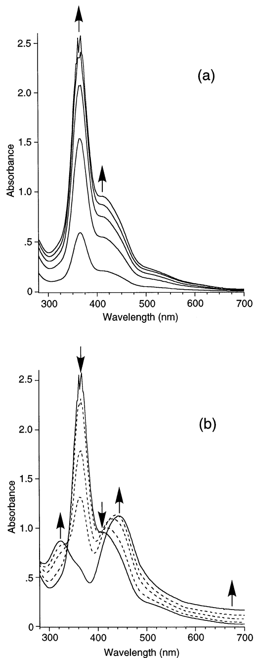
Fig. 6. UV-vis spectral monitoring of the oxygenation of [\text{L}^{\text{iPr}_3}\text{Cu}(\text{CH}_3\text{CN})]\text{PF}_6 (0.28 mM) in THF at -60^\circ\text{C} , (a) every 40 s for the initial 4 min, and (b) after 4 (solid line), 5, 6, 7 (all dashed lines) min, and 20 min (solid line). Adapted from [21].
