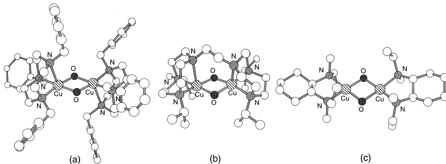
Fig. 3. CHEM3D representations of the cationic portions of the X-ray crystal structures of: (a) [(L^{Bn^3}Cu)_2(\mu-O)_2](SbF_6)_2 [10,14]; (b) [(iPr_4dtne)Cu_2(\mu-O)_2](SbF_6)_2 [ iPr_4dtne = bis(1,4-diisopropyl-1,4,7-triazacyclonon-7-yl)ethane]; and (c) [(L^{ME}Cu)_2(\mu-O)_2](CF_3SO_3)_2 [9a] [ L^{ME} = N,N' -dimethyl- N,N' -diethyl-(1 R ,2 R )-diaminocyclohexane]. Non-carbon atoms are labeled and H atoms are omitted for clarity.
